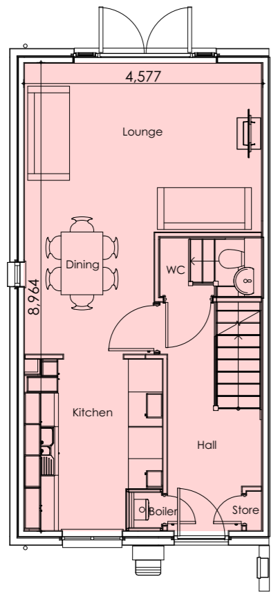
ILKE 3B5P HOUSE GROUND FLOOR PLAN
