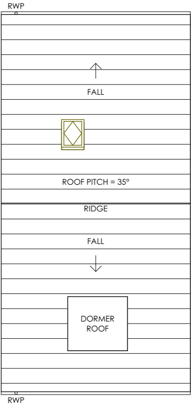
ROOF PLAN
