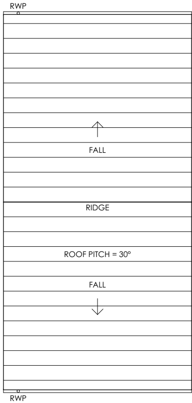
ROOF PLAN
