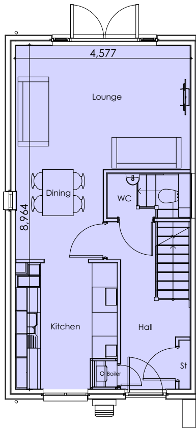
ILKE 2B4P HOUSE GROUND FLOOR PLAN
