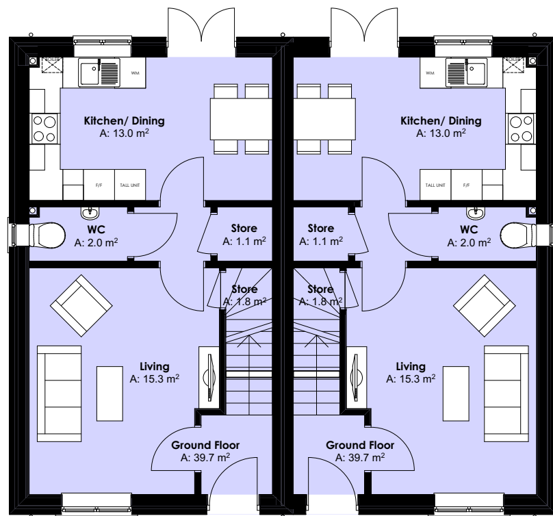
2B4P HOUSE GROUND FLOOR PLAN
